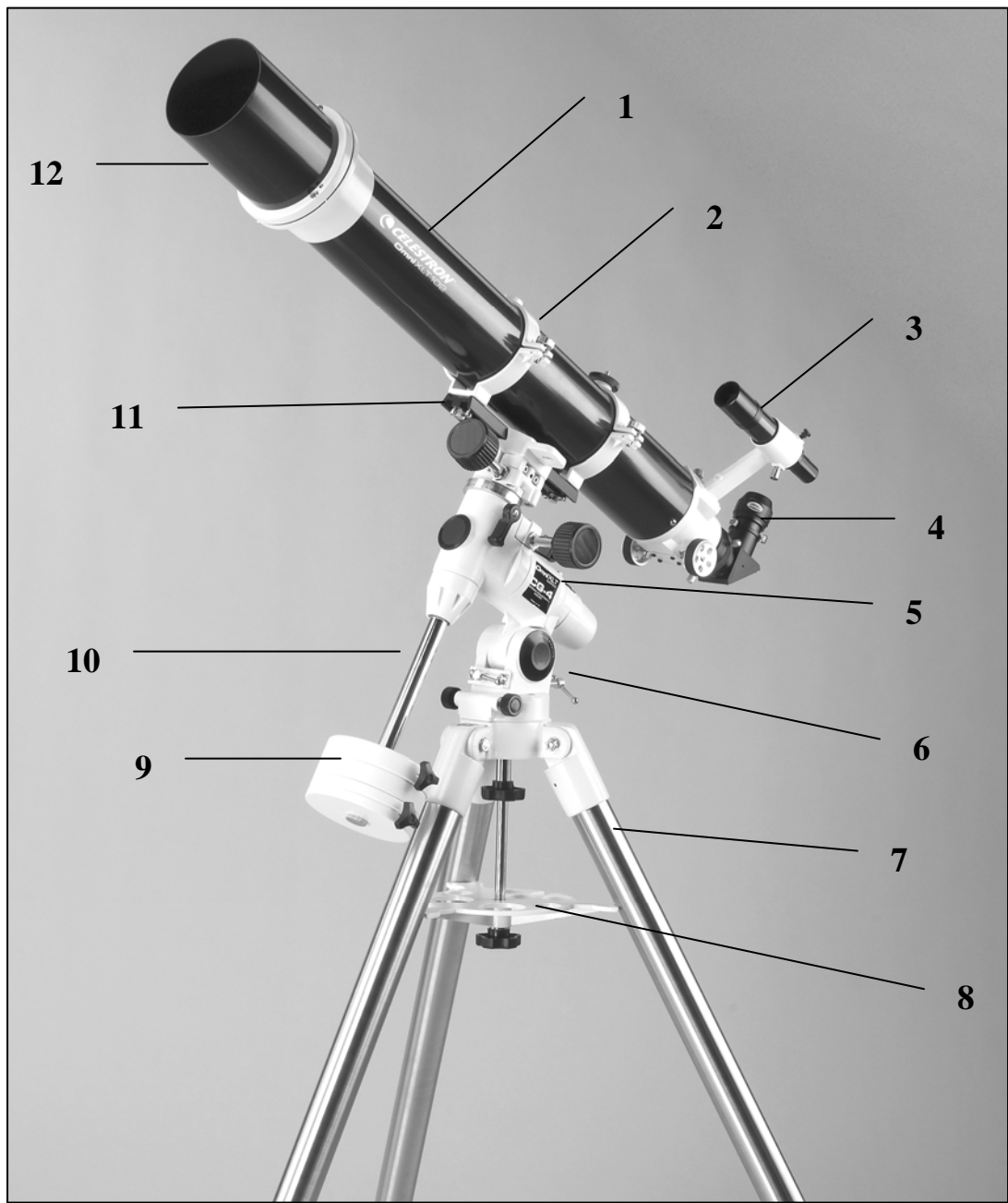
Figure 1-1 Omni XLT 102 Refractor (Omni XLT 120 Refractor similar)
